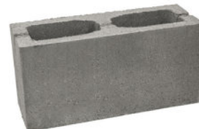
BLOC CREUX 6" 7 1/2" x 5 1/2" x 15 3/8" 190mm x 140mm x 391mm
